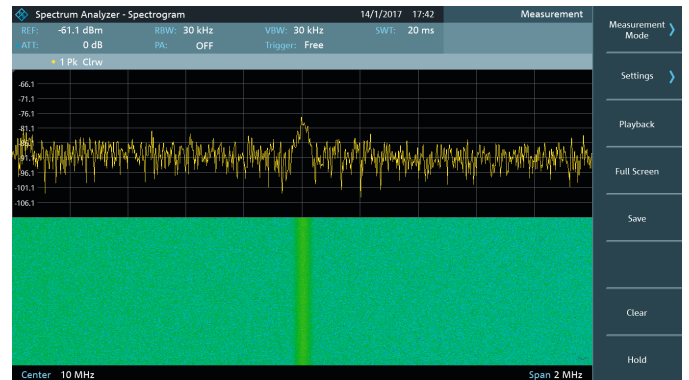
R&S®FPC-K55: spectrogram.
